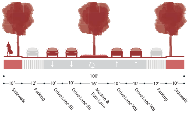
Section B: Proposed Phase I, Area 1 (Figure B.1.e)
