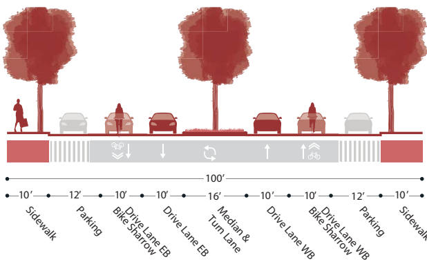
Section D: Proposed Phase 2, Areas 1 and 2 (Full Build-Out) (Figure B.1.h)
