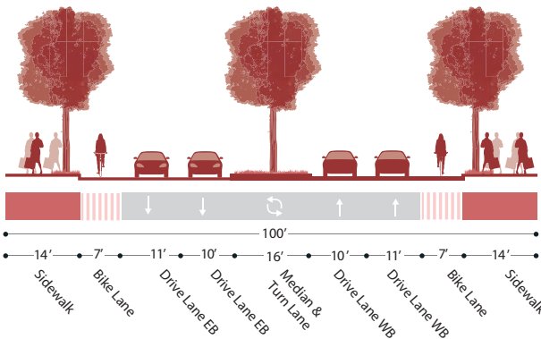
Section D: Proposed Phase 2, Areas 1 and 2 (Full Build-Out) (Figure B.1.h)
