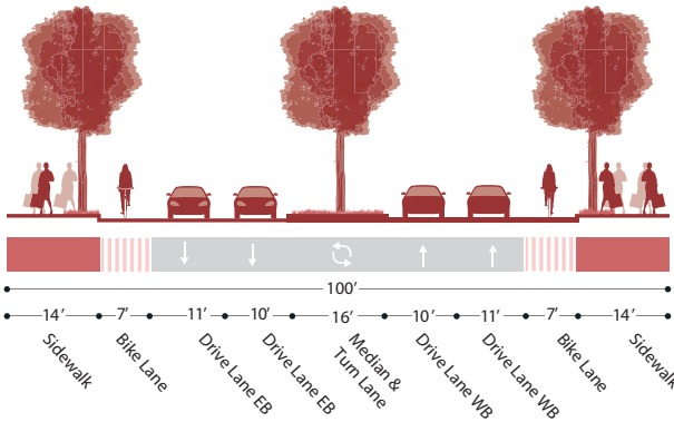
Section C: Proposed Phase I, Area 2 (Figure B.1.f)
